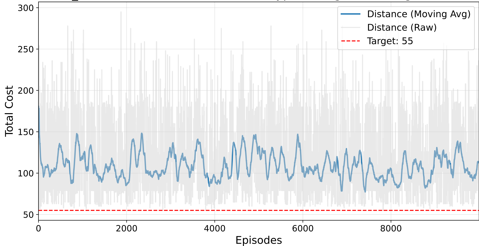
Final NO_BAYESIAN Masked AutoRL-SOP (HyperTuningSK) Training - br17.12.sop
